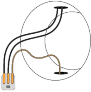
Illustration 9: Connect power to connection terminal on switch 1
