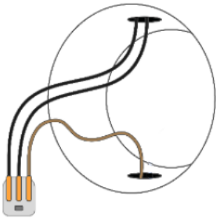
Illustration 6: Connect power to connection terminal
